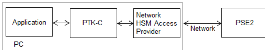
Figure 2: Network Mode using a SafeNet Network HSM
