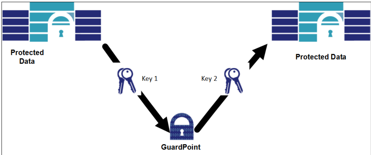
Figure 1-3: Rekeying Protected Data
